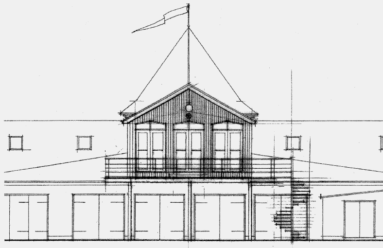
Facade mod fjorden (1:100)
